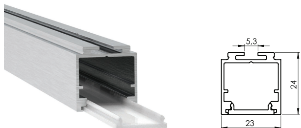
MV-060.1 U - PROFILIS LED 23 X24 (AL LED-SET)
